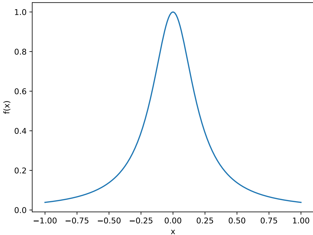
Runge function
