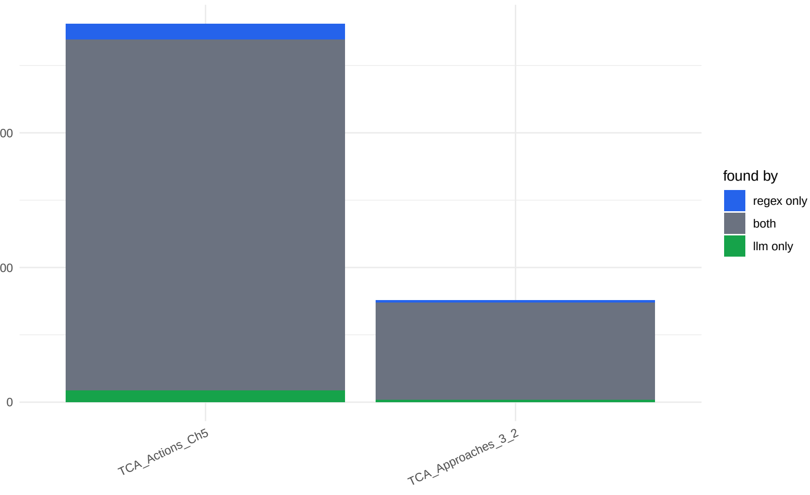
Citation extraction agreement: regex vs LLM, per keyset
