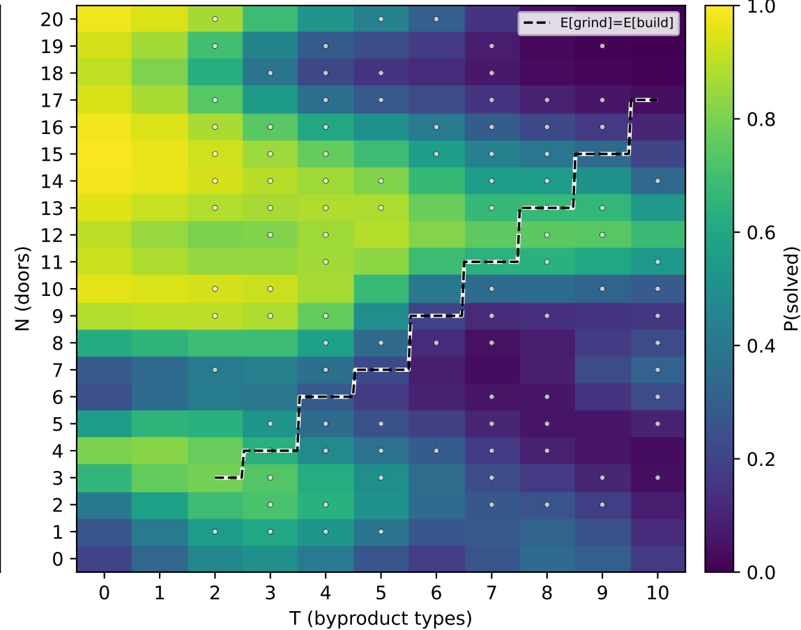
Opus 4.8 (solved 0.46, n=100)
