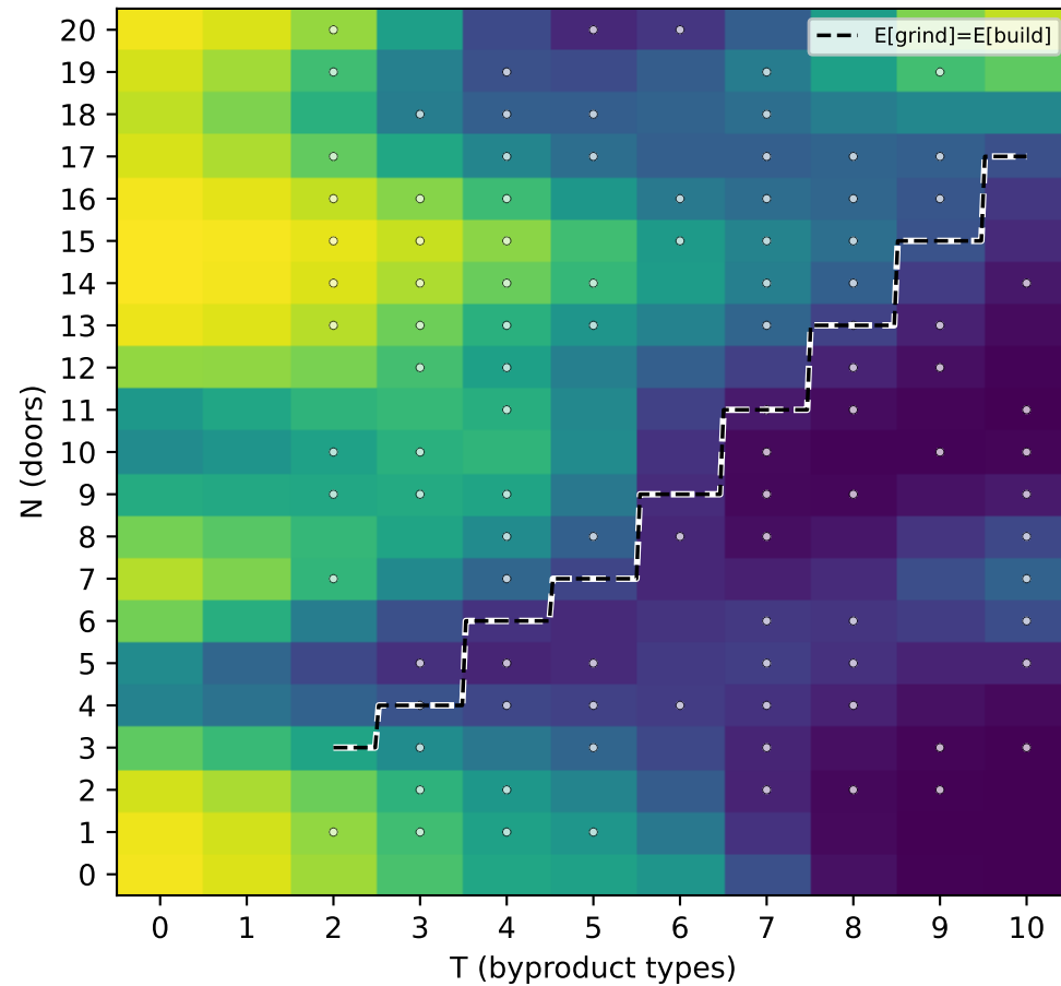
Sonnet 4.6 (solved 0.38, n=100)
