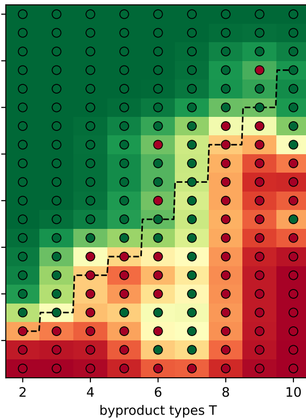
Sonnet held-both rate = 0.63
