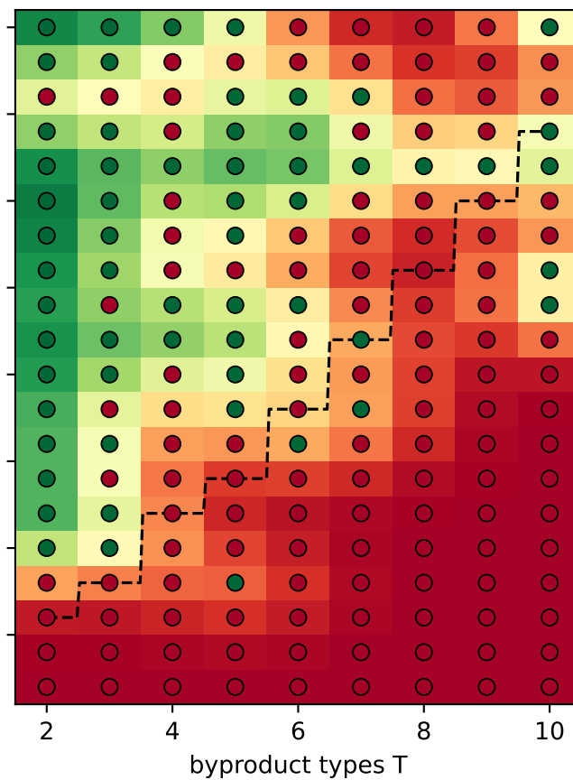
Sonnet solve rate = 0.33
