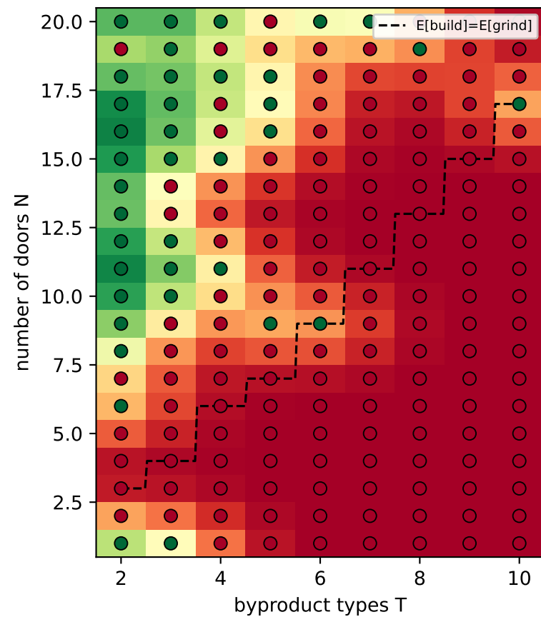
Haiku solve rate = 0.21
