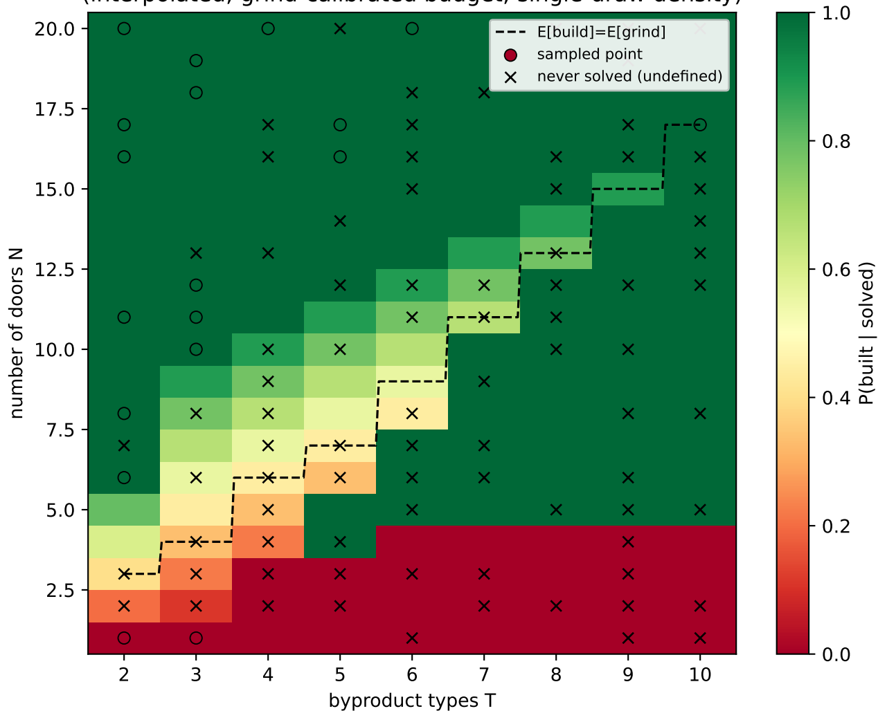
Haiku P(built | solved) over (T, N) (interpolated; grind-calibrated budget; single-draw density)
