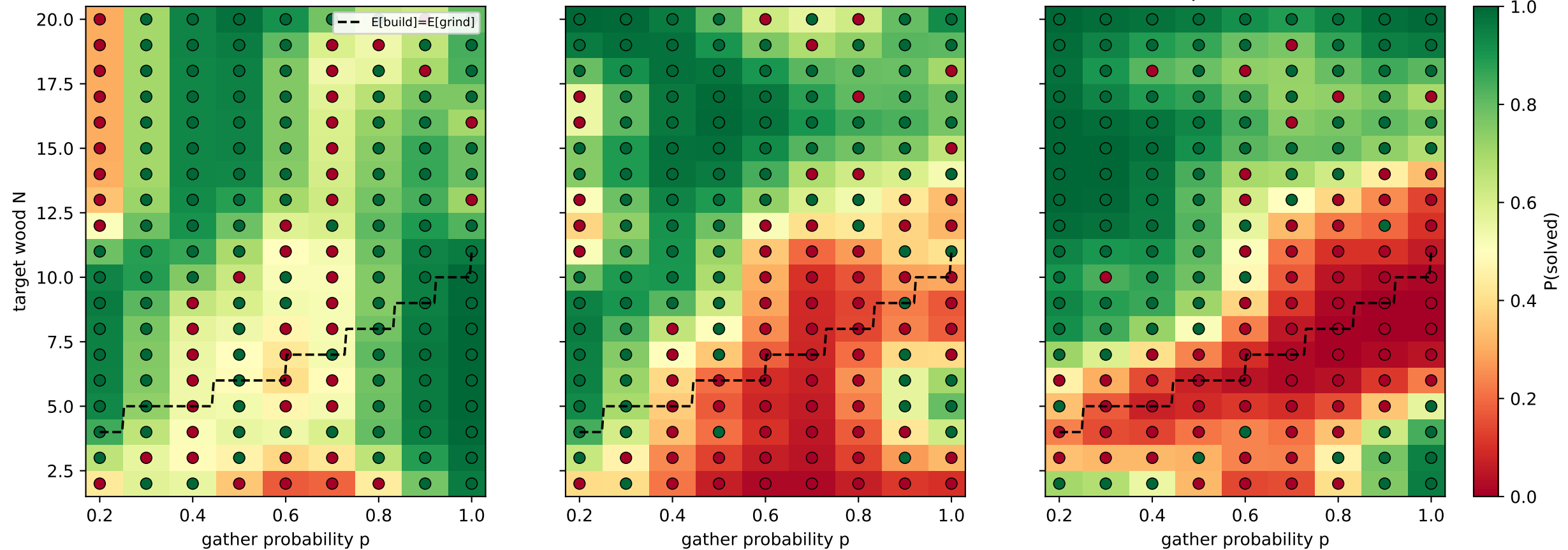
Haiku (0.71)
