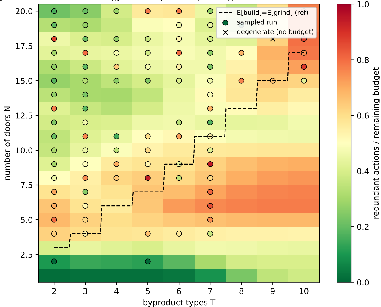
Haiku tool-exploitation efficiency: redundant actions as a fraction of budget after a forced build (gaussian-pooled (bw=1); redundant = no door/machine prod)
