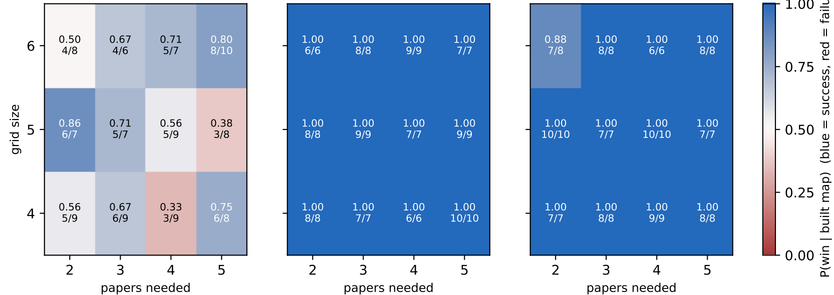
Win rate given the map was built — P(\text{win} \mid \text{built}) , over wins/built
