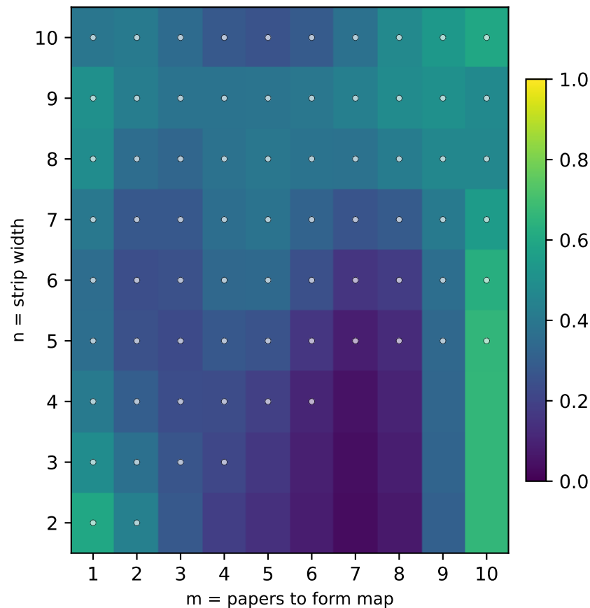
solved (mean 0.35)
