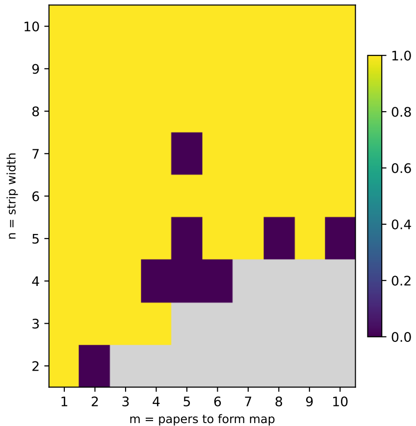
solved (mean 0.89)
