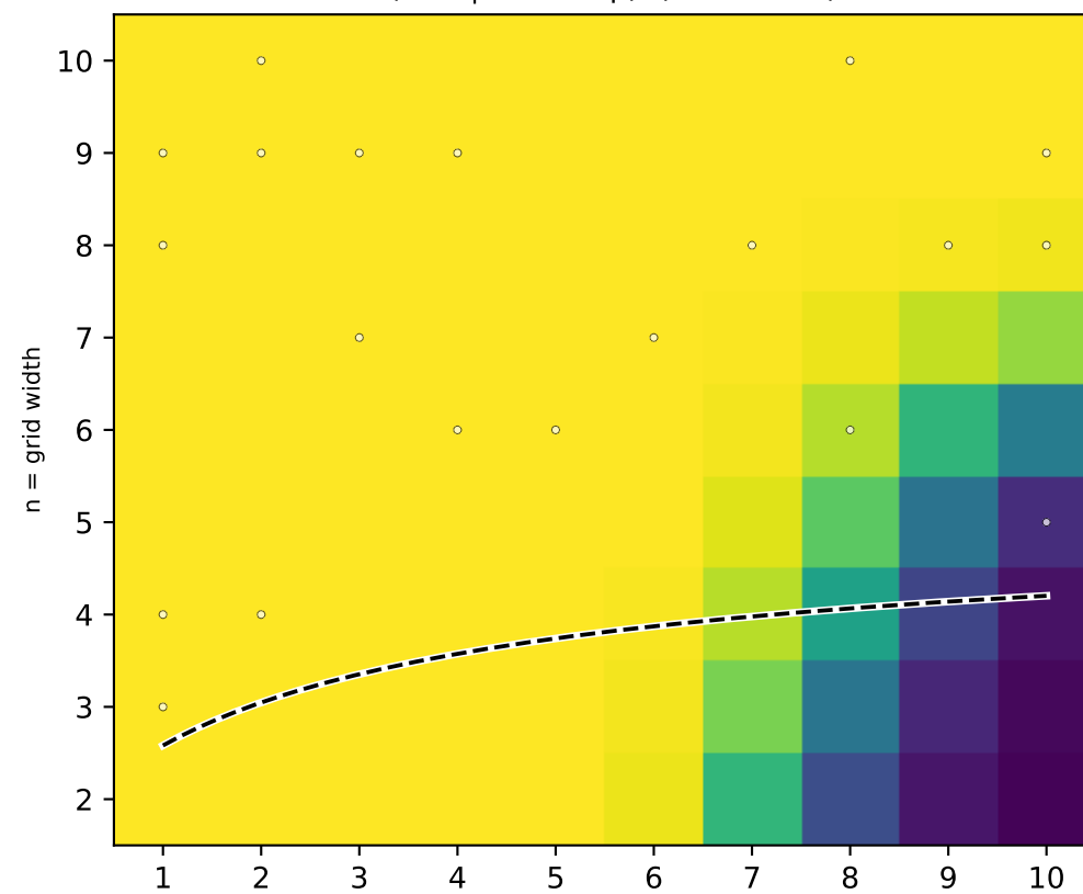
P(won | built map) (mean 0.97)
