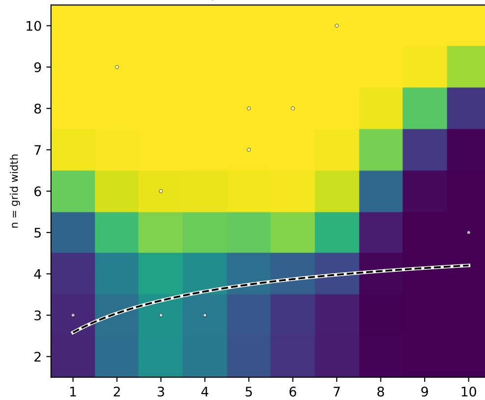
P(won | built map) (mean 0.95)
