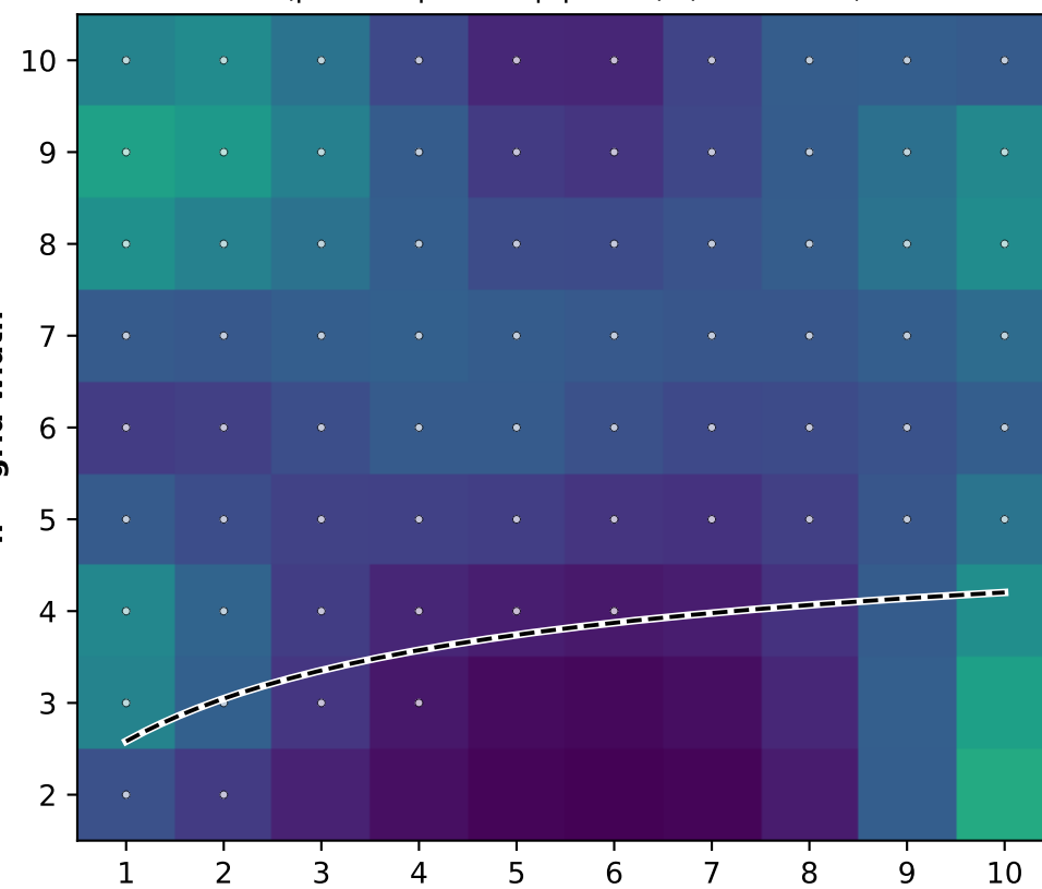
P(picked up all map pieces) (mean 0.89)
