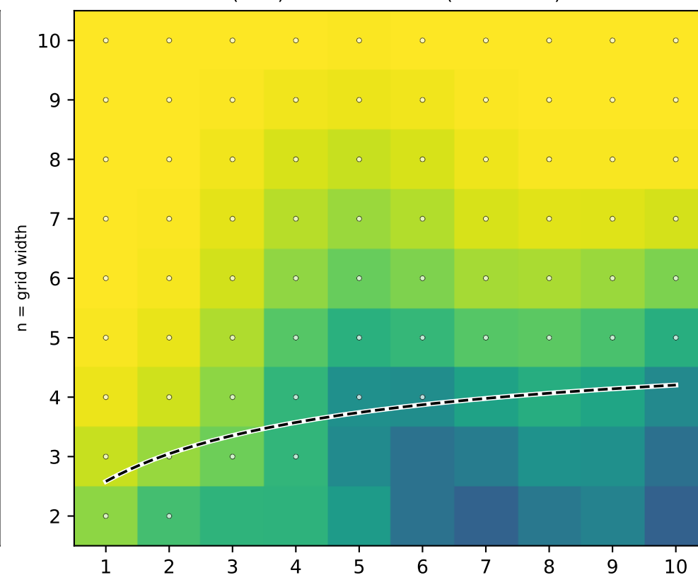
P(won) -- total success (mean 0.89)
