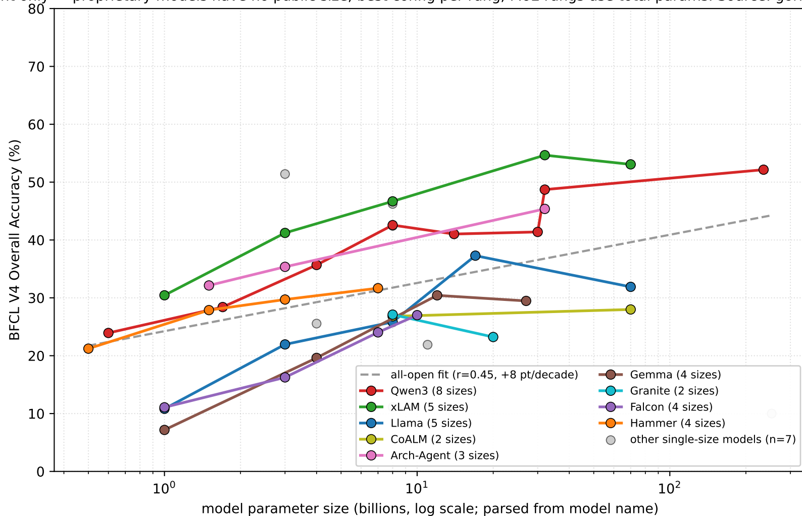
Berkeley Function Calling Leaderboard V4: tool-use accuracy vs. parameter size, by family
