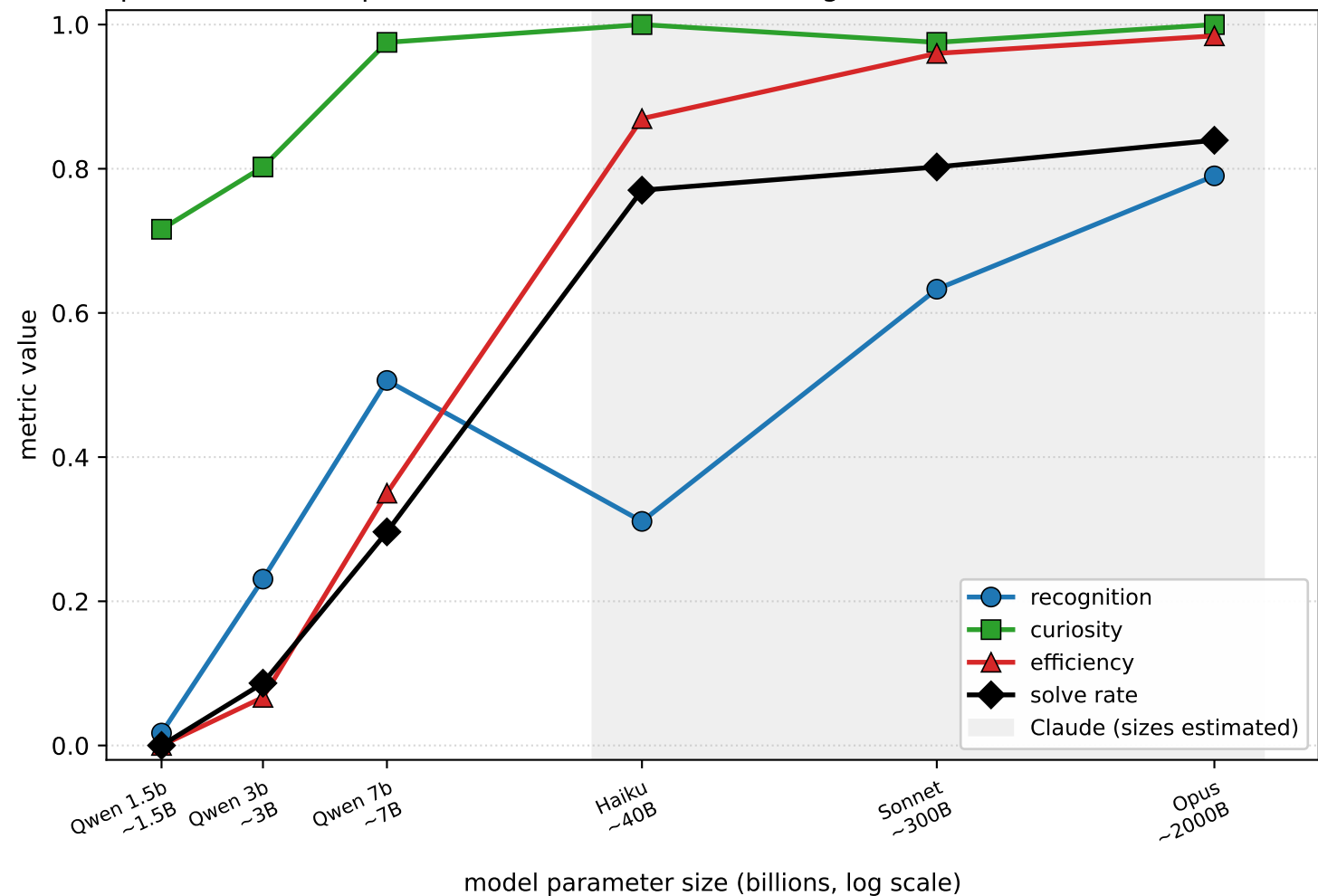
Woodworld: panel metrics vs. model parameter size (pooled headline per model; Claude sizes are rough estimates — see shaded band)
