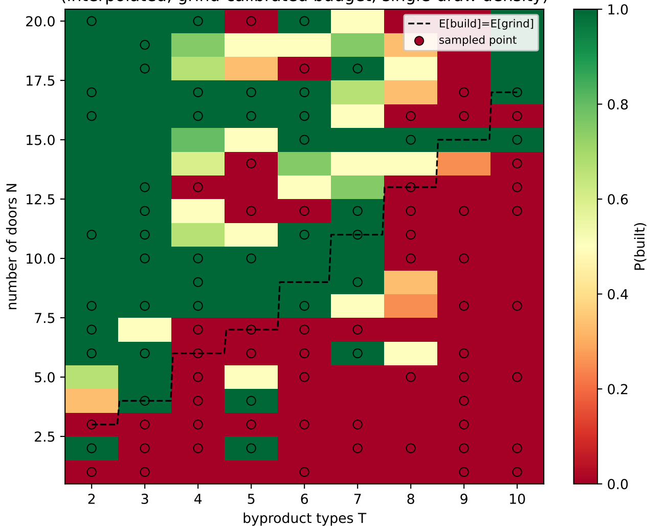
Haiku build-propensity density over (T, N) (interpolated; grind-calibrated budget; single-draw density)
