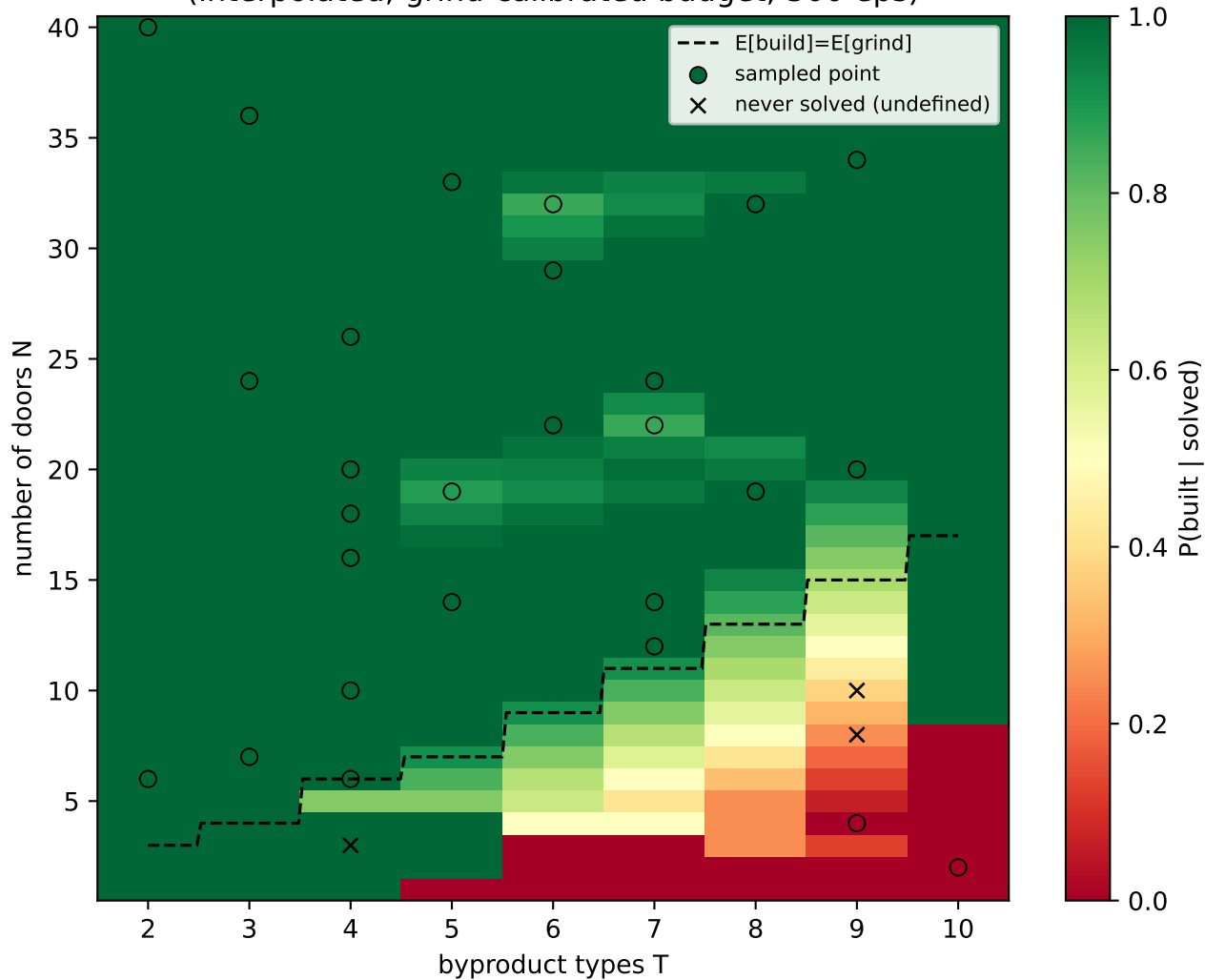
Haiku P(built | solved) over (T, N) (interpolated; grind-calibrated budget; 300 eps)
