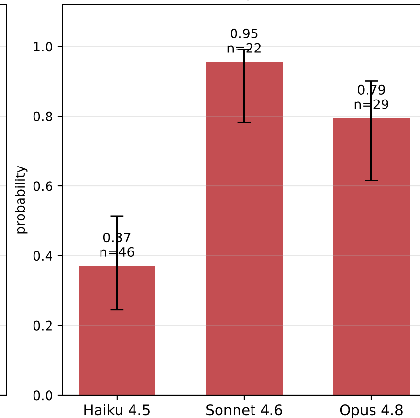
P(won | built)
