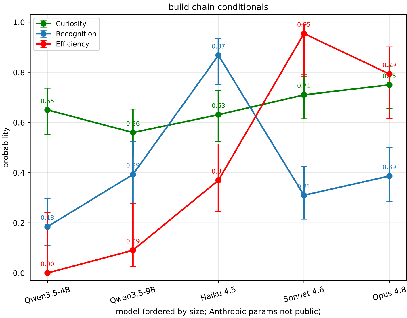
toolworld v3 vs model size (proportion over sampled N,T cells, T \geq 2 ; bars = Wilson 95% CI)
