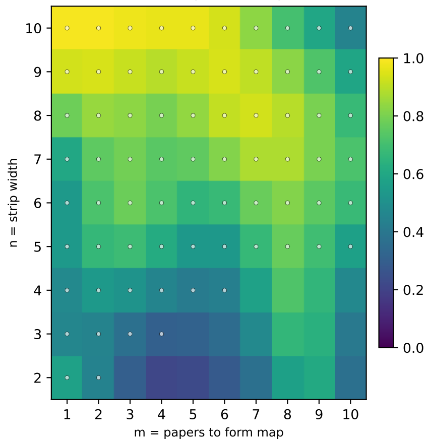
solved (mean 0.72)
