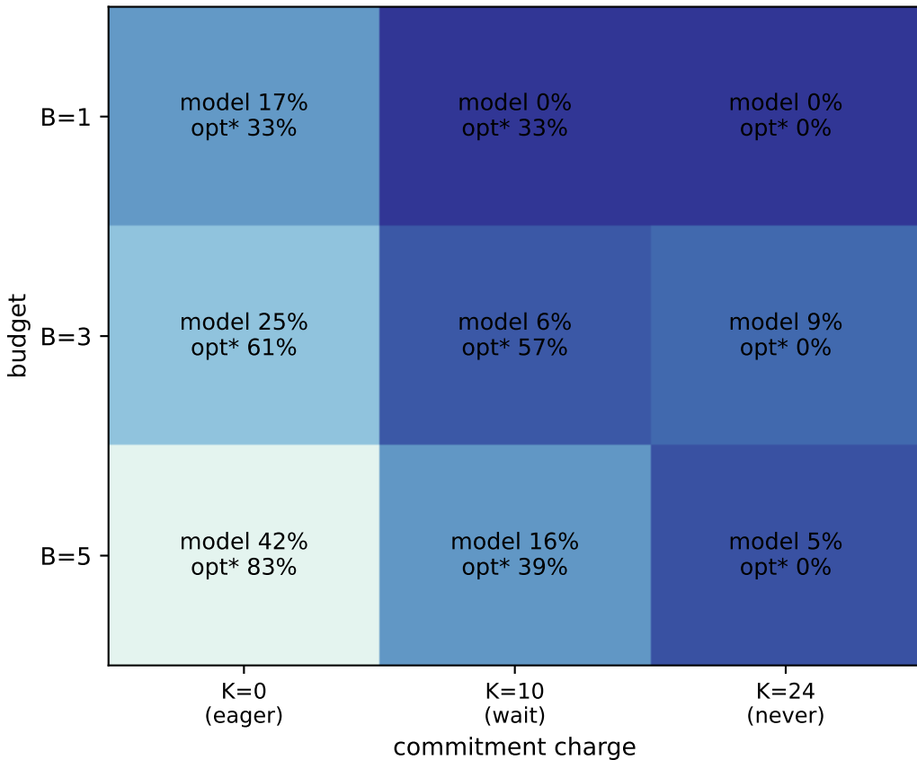
R0 (abstract free-text keep/pass)
