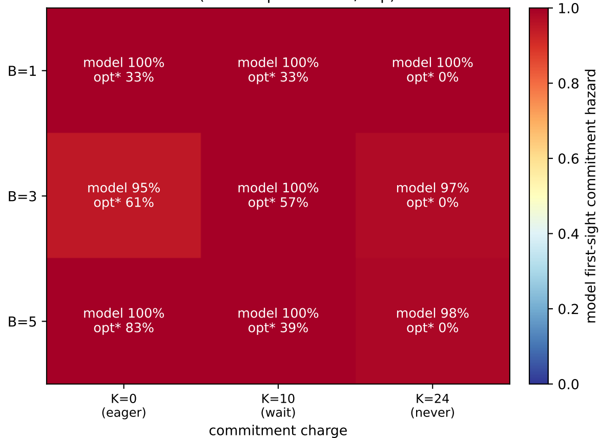
R2c (code-required claim/skip)
