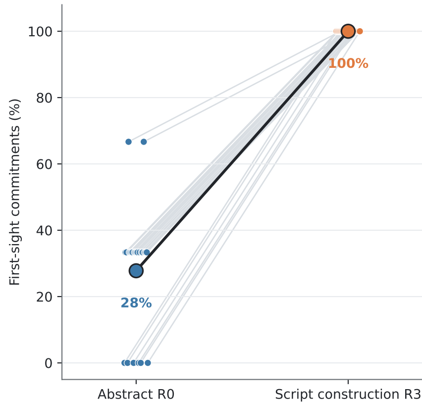
b Same-information Haiku dissociation
