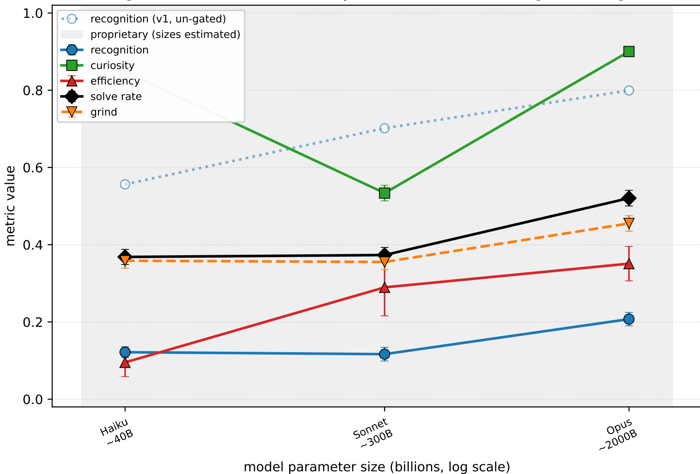
CREATOR v3 (visible batch, announced ~400-tok budget): C·R·E vs model size Recognition = P(built reusable tool | asked); dashed = v1 recognition (un-gated)
