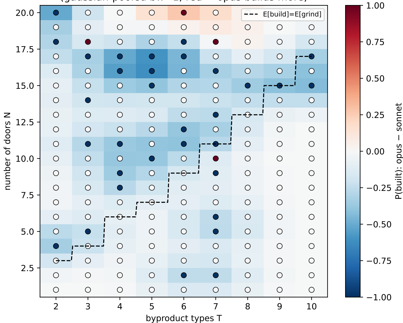
Build-propensity difference: Opus – Sonnet (gaussian-pooled bw=1; red = opus builds more)
