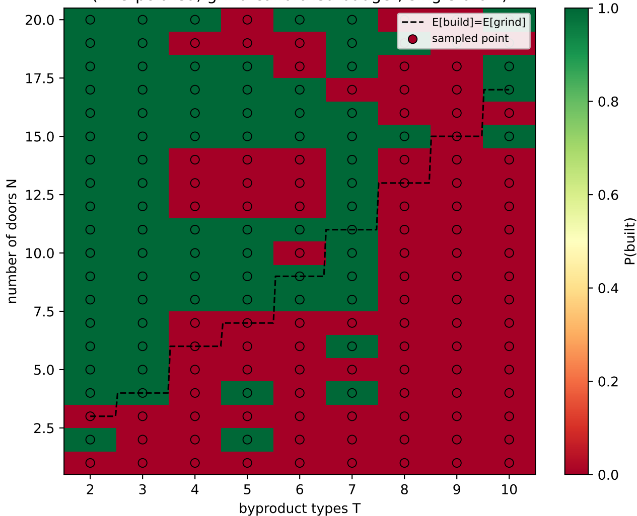
Haiku build-propensity density over (T, N) (interpolated; grind-calibrated budget; single-draw)
