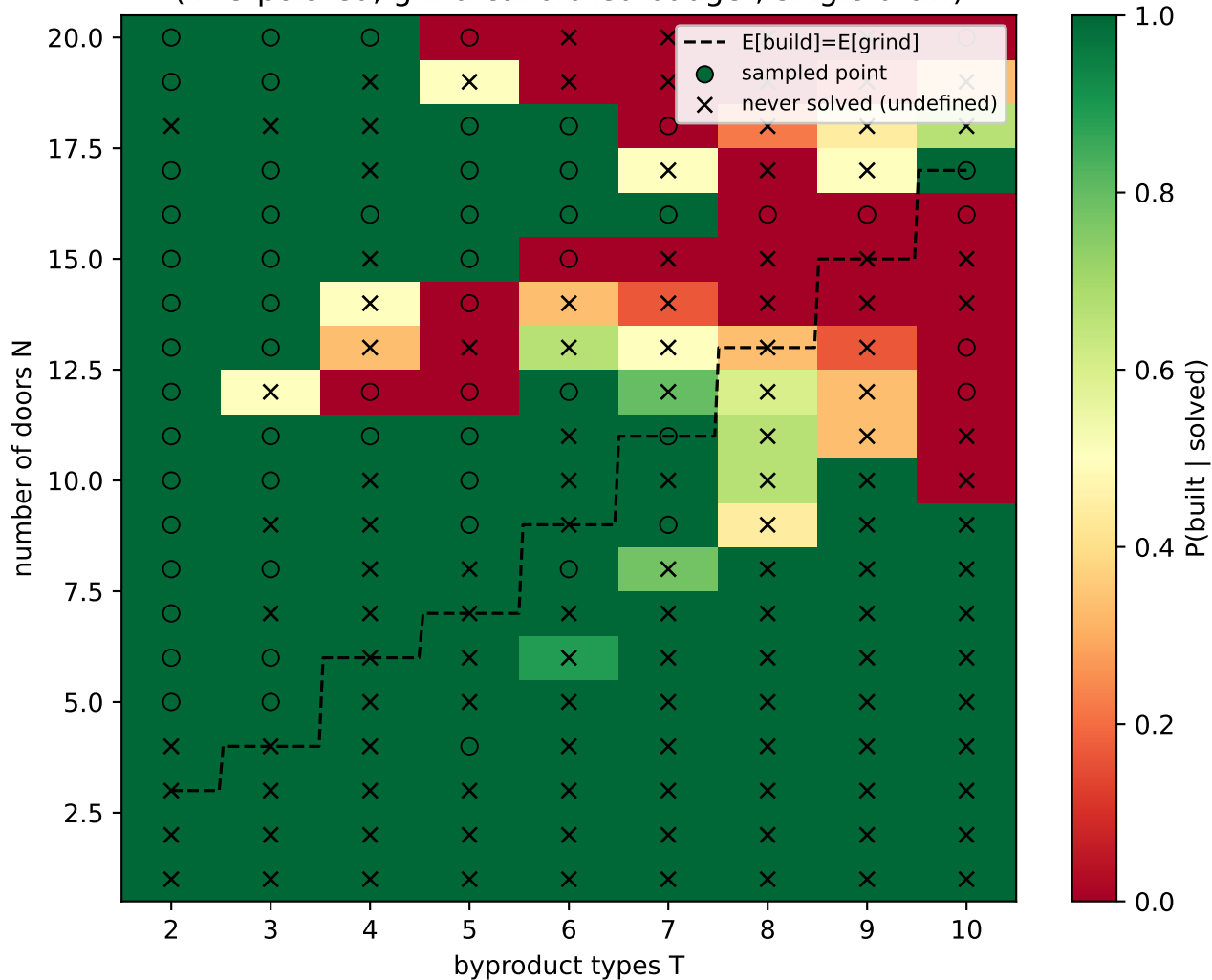
Sonnet P(built | solved) over (T, N) (interpolated; grind-calibrated budget; single-draw)
