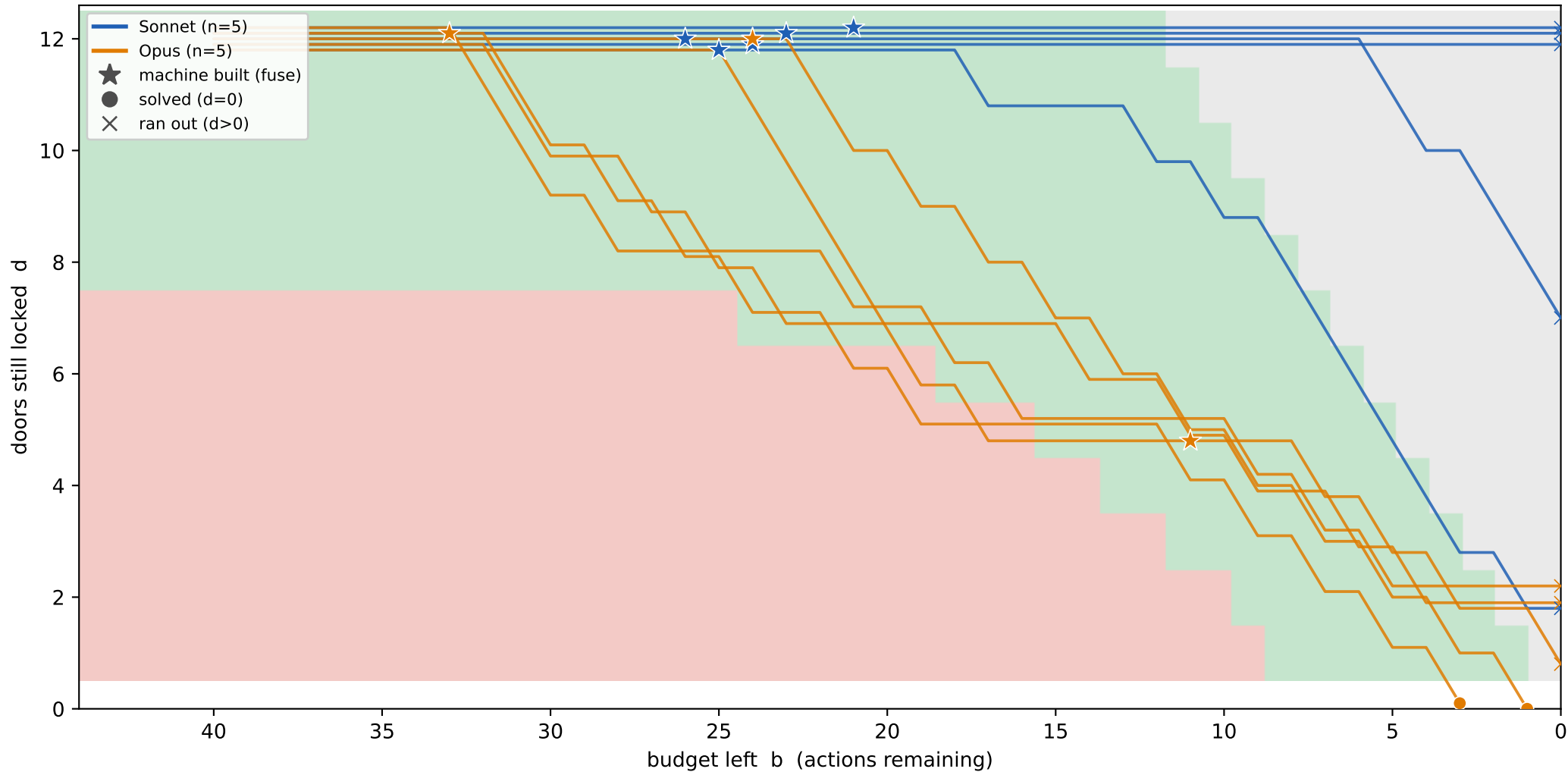
Episode trajectories on the MDP policy map (start b=40 , d=12 ; T=3 ) green=grind region, red=build region, grey=hopeless
