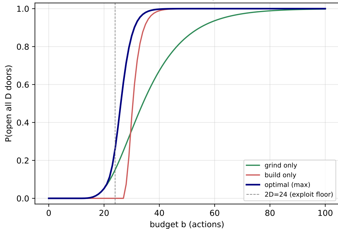
Start state success vs budget (D=12, T=3)
