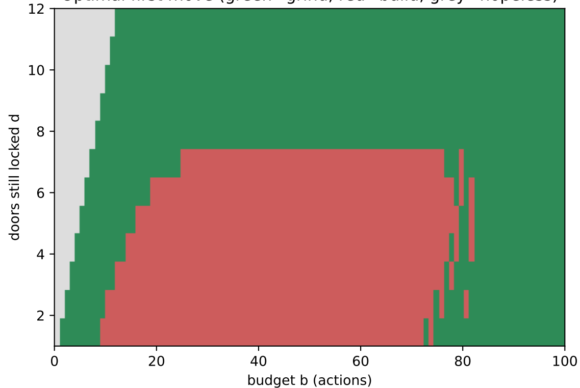
Optimal first move (green=grind, red=build, grey=hopeless)
