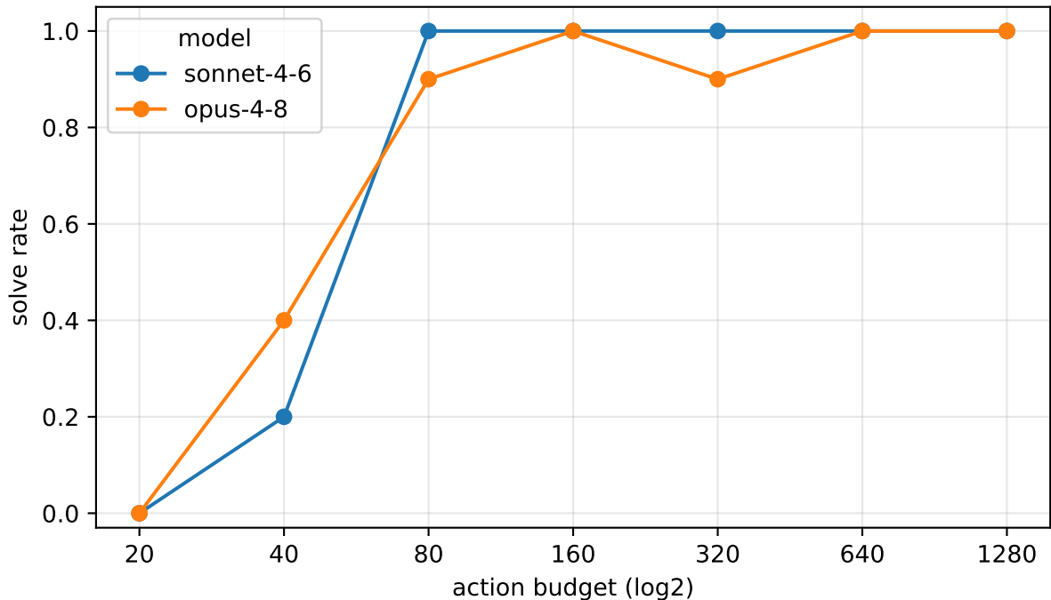
Solve rate vs. budget (n=12, T=3, 10 reps/cell)
