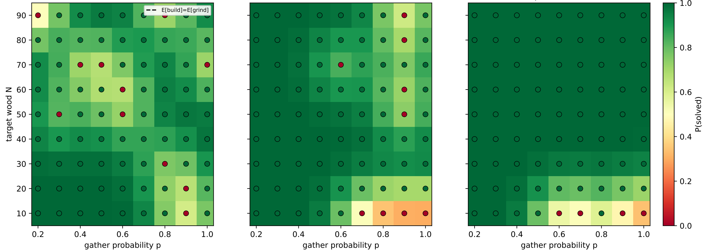
Haiku (0.86)
