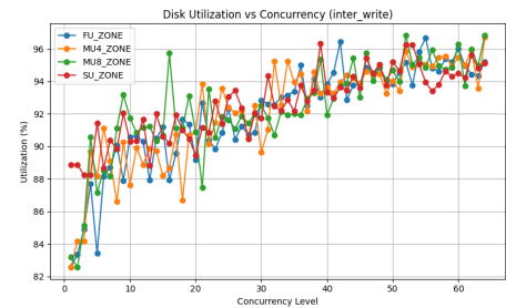
Figure 13: Utilization vs Concurrency Inter Write
