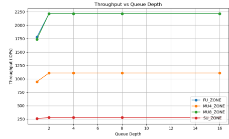
Figure 11: Intra Zone Throughput
