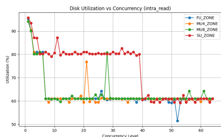
Figure 14: Utilization vs Concurrency Intra Read
