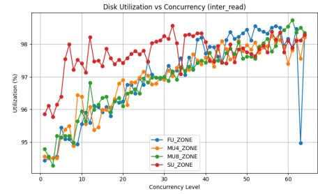
Figure 12: Utilization vs Concurrency Inter Read
