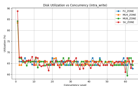
Figure 15: Utilization vs Concurrency Intra Write
