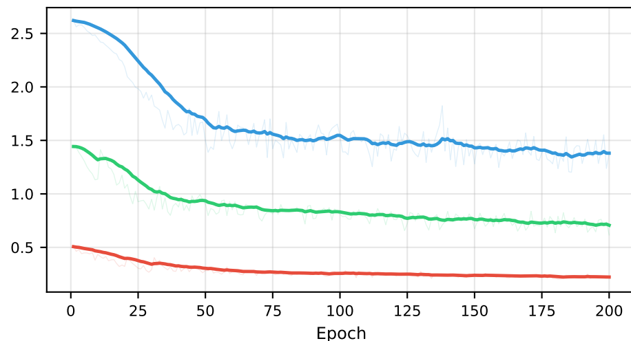
Conservative Penalty
