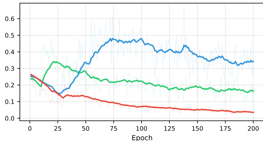
Mean Q-Value
