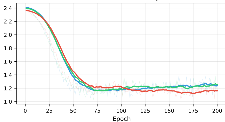
Conservative Penalty
