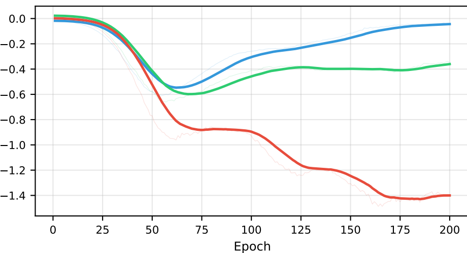
Mean Q-Value
