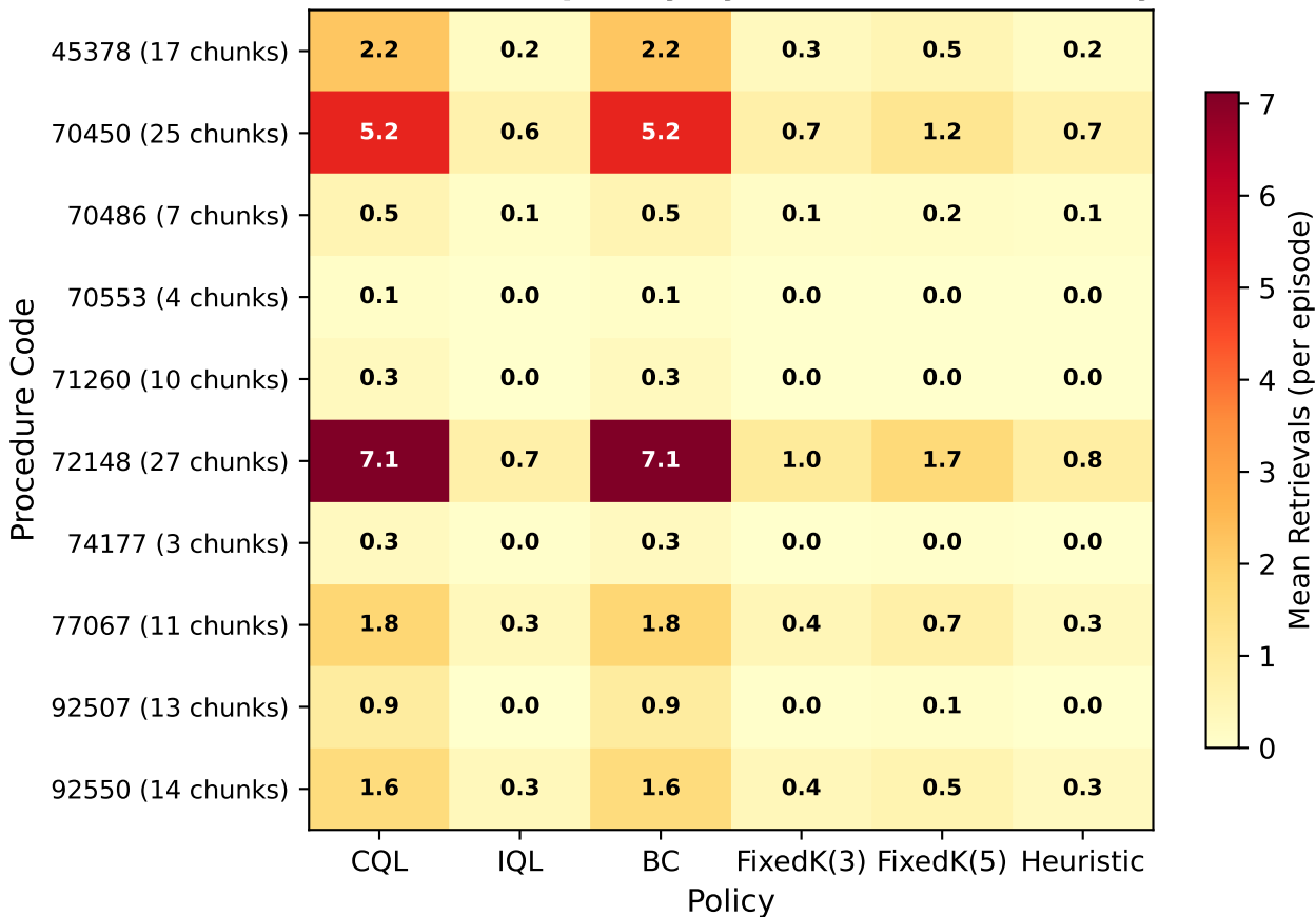
Retrieval Frequency by Procedure and Policy
