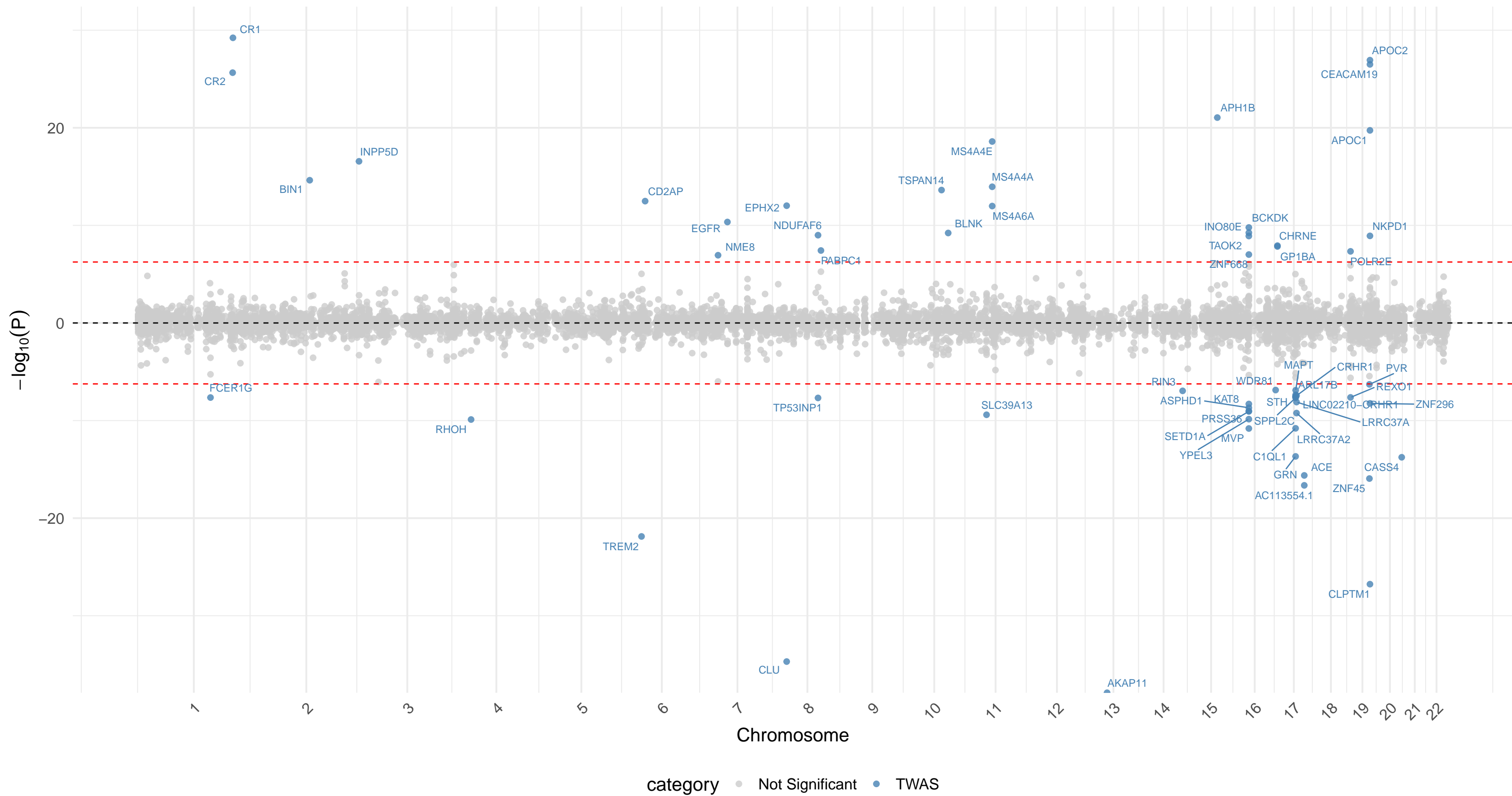
Manhattan Plot of TWAS for AD_Bellenguez_2022 in DLPFC bulk RNA-seq
