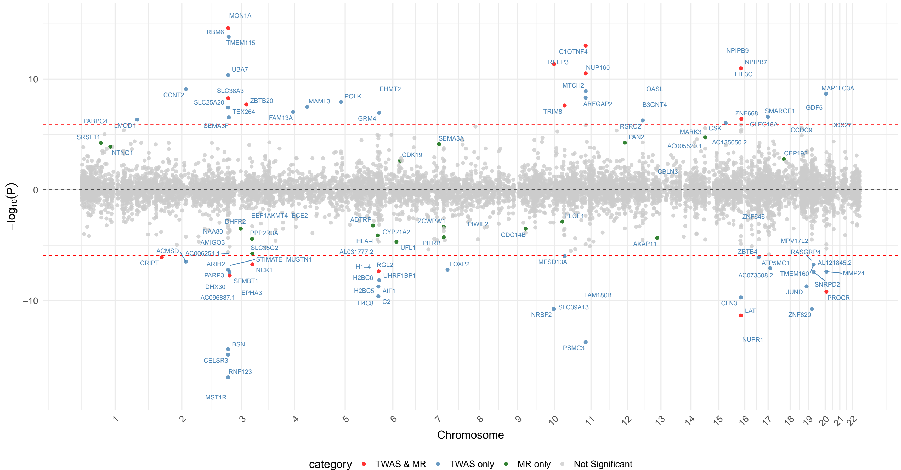
Manhattan Plot of TWAS for unadjusted self-reported walking pace in DLPFC
