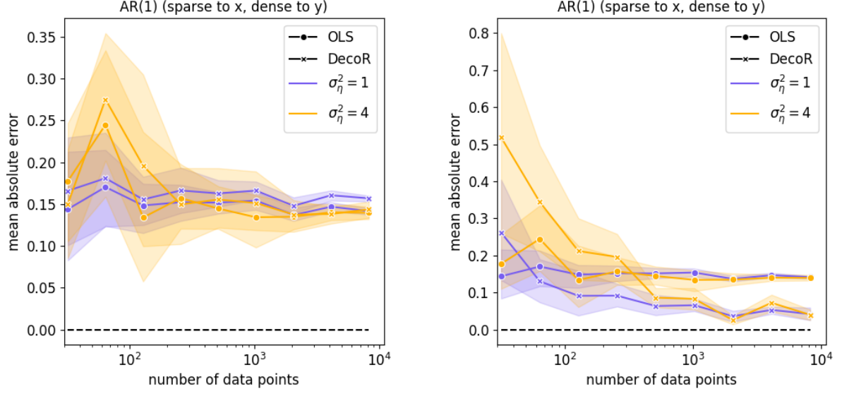
Figure 3: Comparison of original and modified DecoR-Torrent in the new scenario. Left: OLS vs original DecoR-Torrent, Right: OLS vs modified DecoR-Torrent. The simulated AR(1)-process follows the parametrization of Sec. 2.
