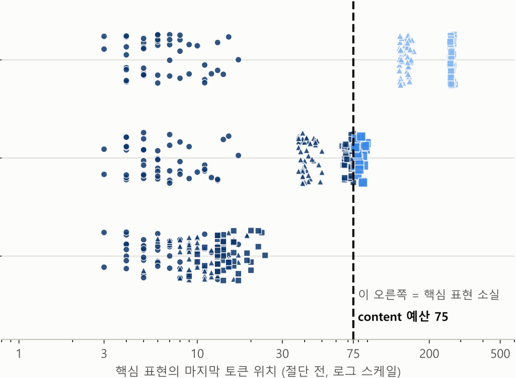
B AltDiffusion native (content 예산 75)
