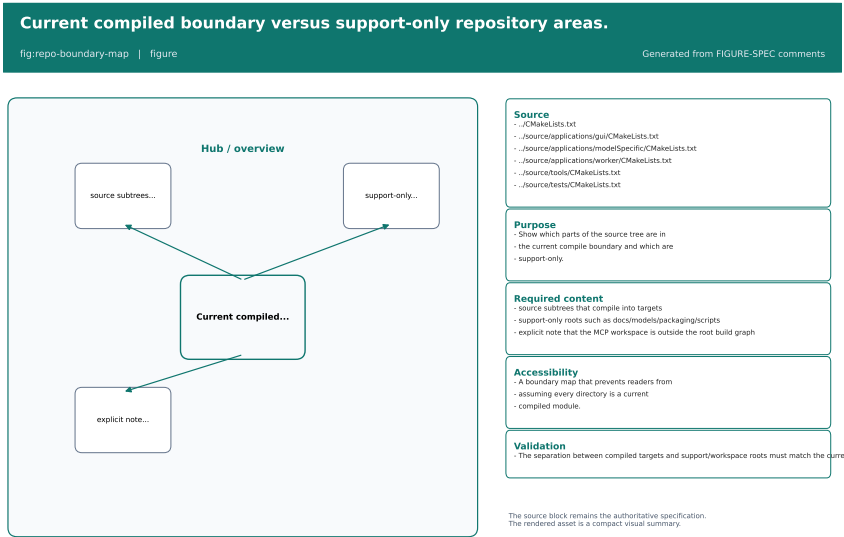
Figure 15.4: Current compiled boundary versus support-only repository areas.
