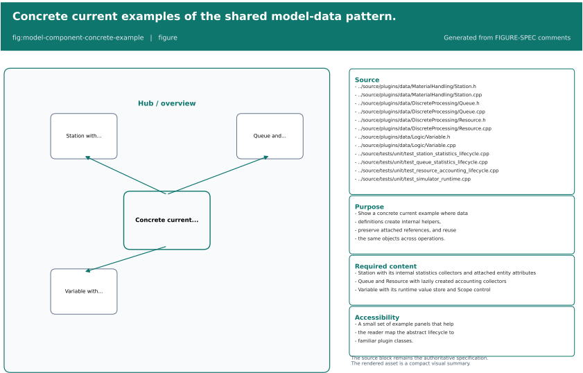
Figure 19.5: Concrete current examples of the shared model-data pattern.
