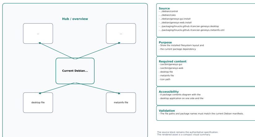
Figure 31.4: Current Debian package contents and install layout.
