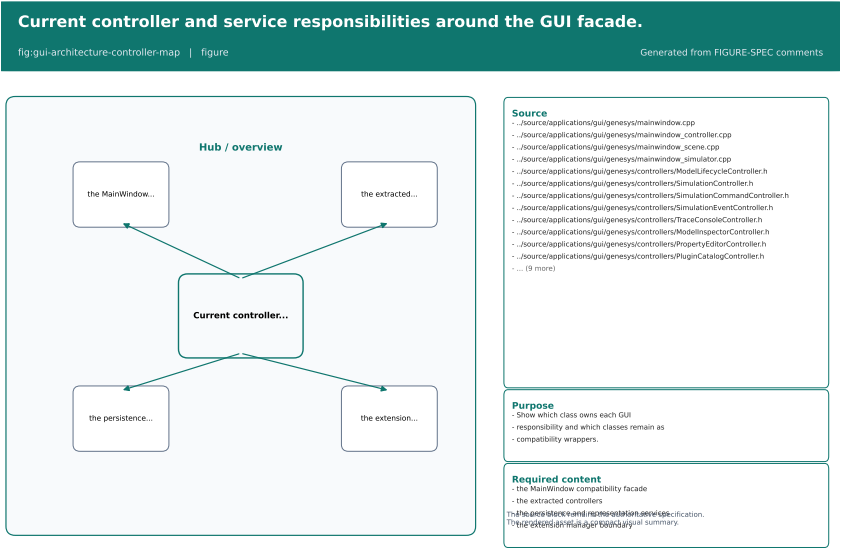
Figure 26.2: Current controller and service responsibilities around the GUI facade.
