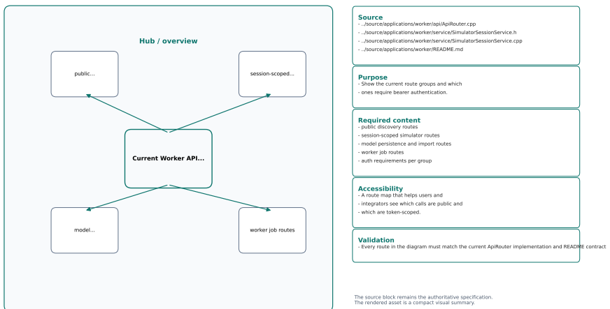
Figure 27.4: Current Worker API surface and authentication boundary.
