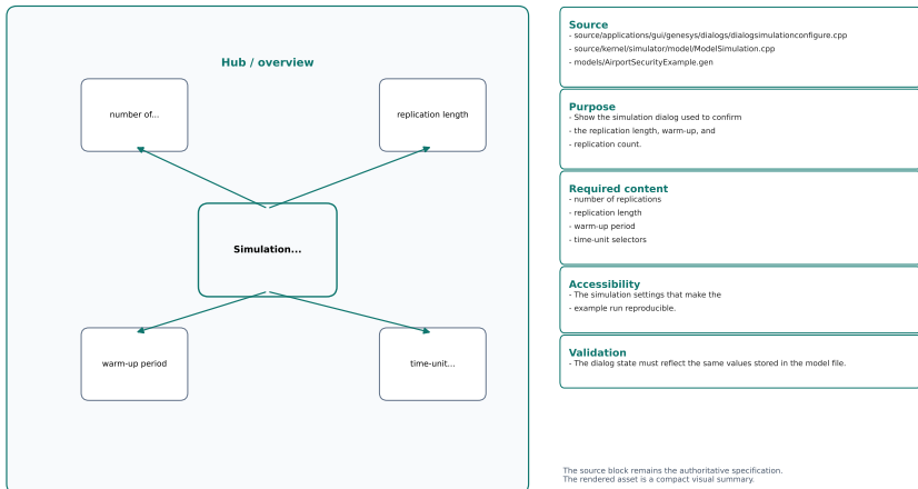
Figure 4.4: Simulation configuration for the baseline tutorial run.
