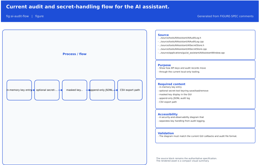
Figure 28.5: Current audit and secret-handling flow for the AI assistant.
