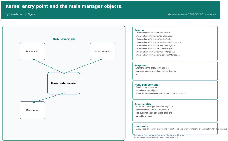
Figure 16.1: Kernel entry point and the main manager objects.
