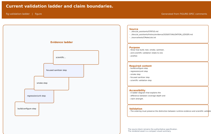
Figure 30.3: Current validation ladder and claim boundaries.
