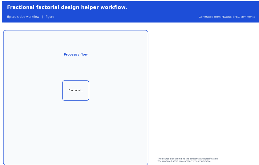
Figure 23.4: Fractional factorial design helper workflow.
