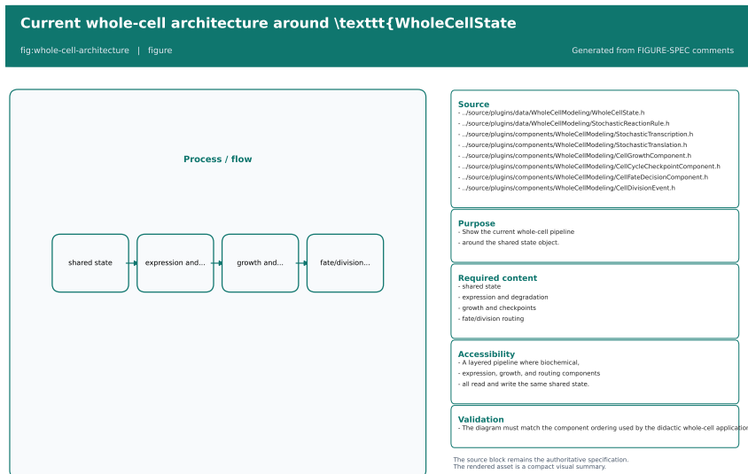
Figure 29.4: Current whole-cell architecture around WholeCellState .
