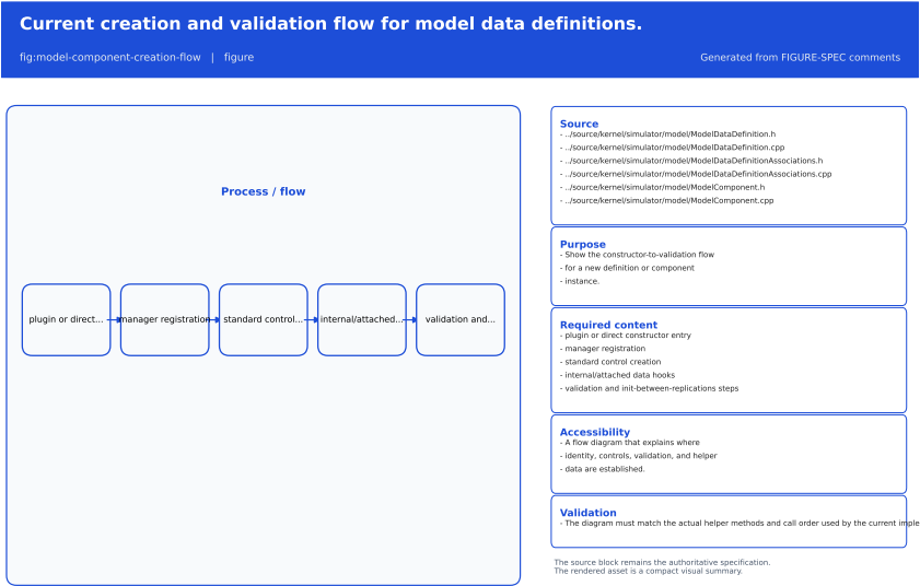
Figure 19.3: Current creation and validation flow for model data definitions.
