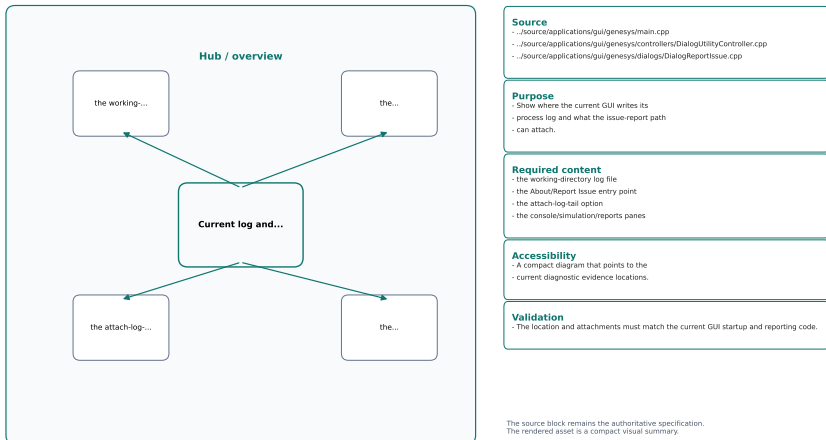
Figure 13.4: Current log and reporting locations.
