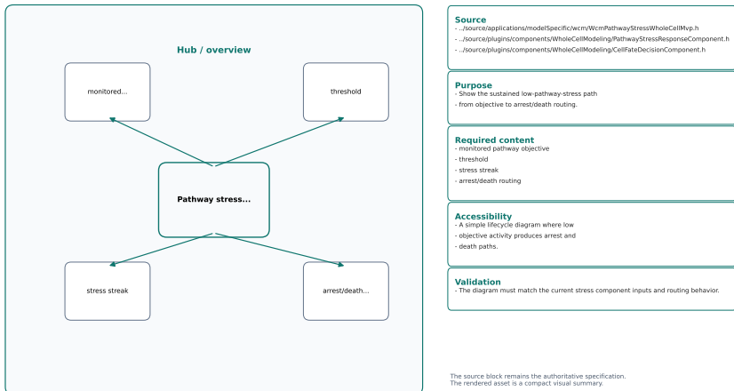
Figure 29.6: Pathway stress example in the current whole-cell surface.
