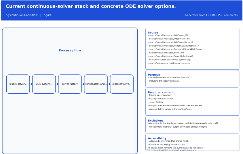
Figure 24.1: Current continuous-solver stack and concrete ODE solver options.
