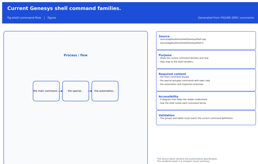
Figure 9.2: Current Genesys shell command families.
