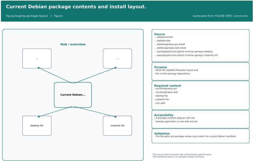
Figure 31.4: Current Debian package contents and install layout.
