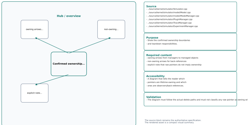
Figure 16.2: Confirmed ownership and back-reference boundaries in the kernel.
