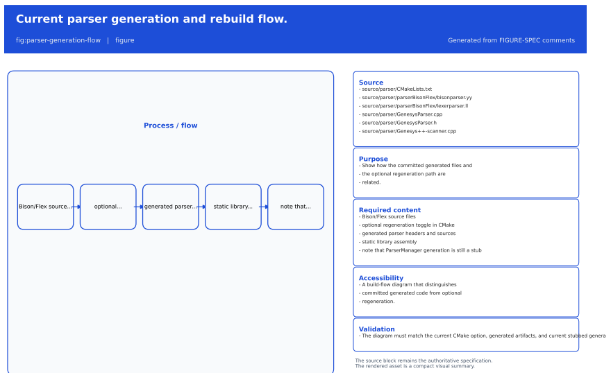
Figure 21.3: Current parser generation and rebuild flow.
