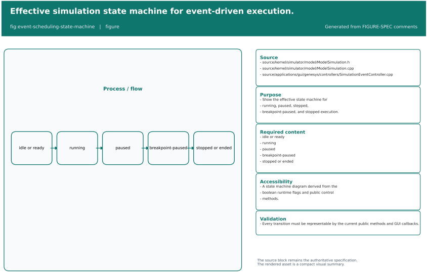
Figure 17.4: Effective simulation state machine for event-driven execution.
