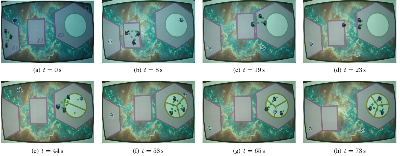
Fig. 2. Snapshots of the hardware-in-the-loop experiment in the hypothetical interstellar exploration mission using three differential-drive wheeled robots, where the extraterrestrial environment is represented through projected scenes. The purple zones Z1, Z2, and Z3 represent the safe zones in which the robots must remain to prevent entry into the plasma fields. The two blue circular regions with lightning represent the electromagnetic storms. When two robots are connected, a green dashed line appears between them. The highland, with a higher density of extraterrestrial flora and fauna, is enclosed by the gray circle. This circle turns orange when at least two robots reach the highland. The orange lines in the highland represent the boundaries of the Voronoi cells of the robots and the orange dots represent their corresponding centers of mass, i.e., optimal coverage locations.
