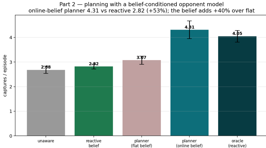
Figure 2: Planning with a belief-conditioned opponent model. The online-belief planner tops every reactive policy, including the oracle; ablating the belief to flat removes most of the gain, isolating the inferred opponent model as the source of the improvement.
