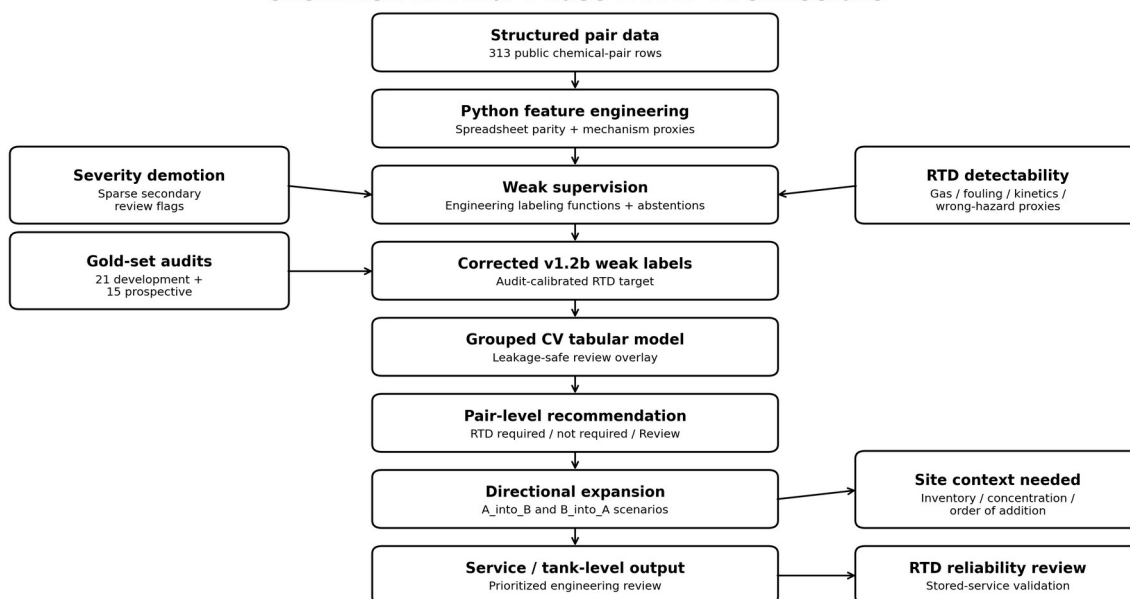
Figure 1. Final ChemRisk-AI Phase 1 MVP architecture. The final workflow uses mechanism-aware weak labels, audit-calibrated v1.2b RTD decisions, targeted LF17/LF18 chemistry-pathway updates, leakage-safe grouped cross-validation, model-assisted review routing, directional A_into_B / B_into_A scenario expansion, and stored-service RTD reliability review before final service-level recommendations.
