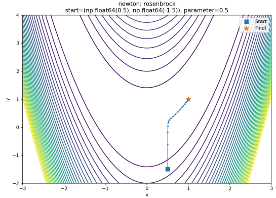
Fig. 12. Newton's Method on the Rosenbrock function
