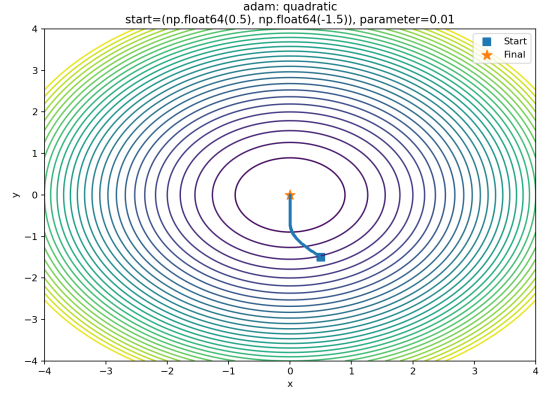
Fig. 5. ADAM on the Quadratic function
