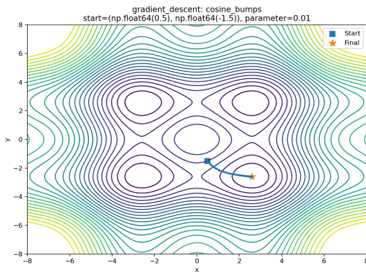
Fig. 7. Gradient Descent on the Cosine Bumps function
