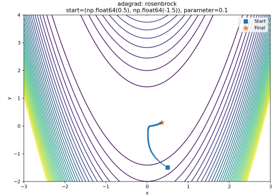
Fig. 3. Adagrad on the Rosenbrock function
