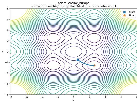
Fig. 4. ADAM on the Cosine Bumps function
