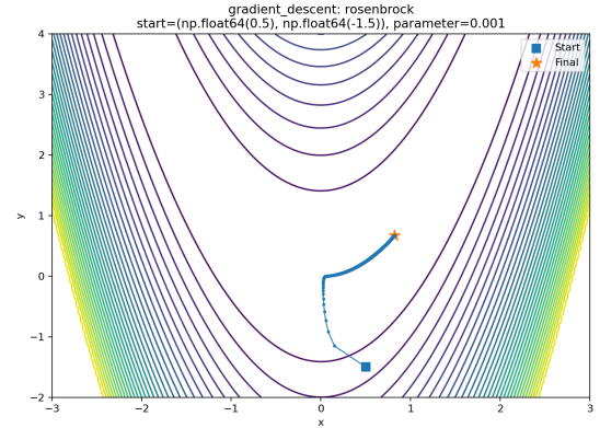
Fig. 9. Gradient Descent on the Rosenbrock function
