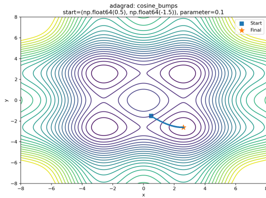
Fig. 1. Adagrad on the Cosine Bumps function
