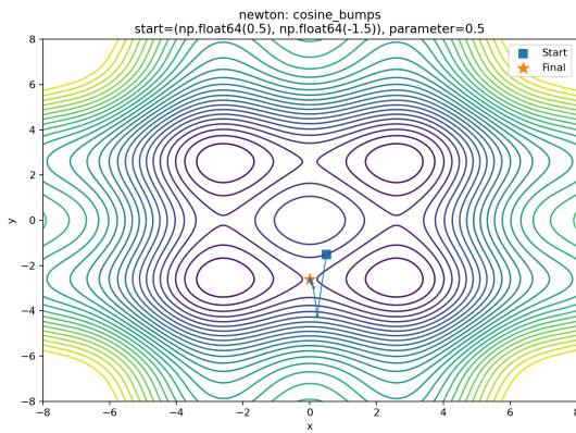
Fig. 10. Newton's Method on the Cosine Bumps function
