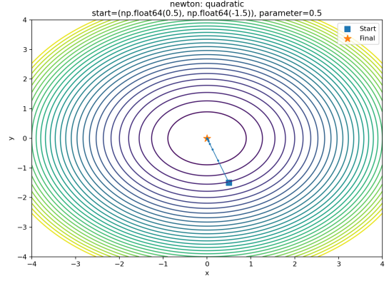
Fig. 11. Newton's Method on the Quadratic function
