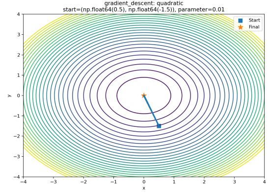
Fig. 8. Gradient Descent on the Quadratic function
