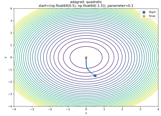
Fig. 2. Adagrad on the Quadratic function
