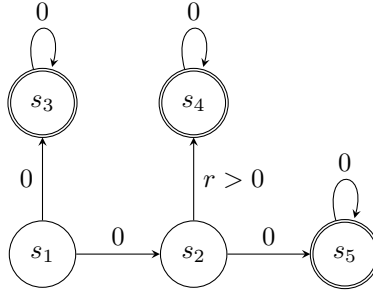
Figure 9.1: (Non-concavity example) A deterministic MDP corresponding to Lemma 9.7 where V^{\pi_\theta}(s) is not concave. Numbers on arrows represent the rewards for each action.
