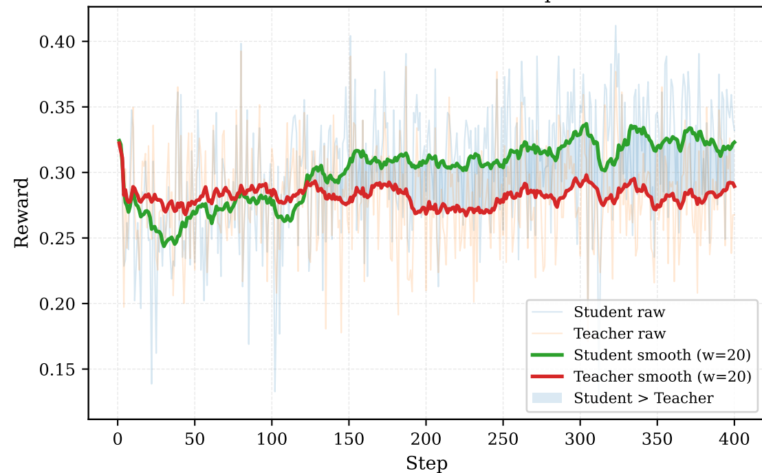
5-NFE - Reward Gap (Student - Teacher)
