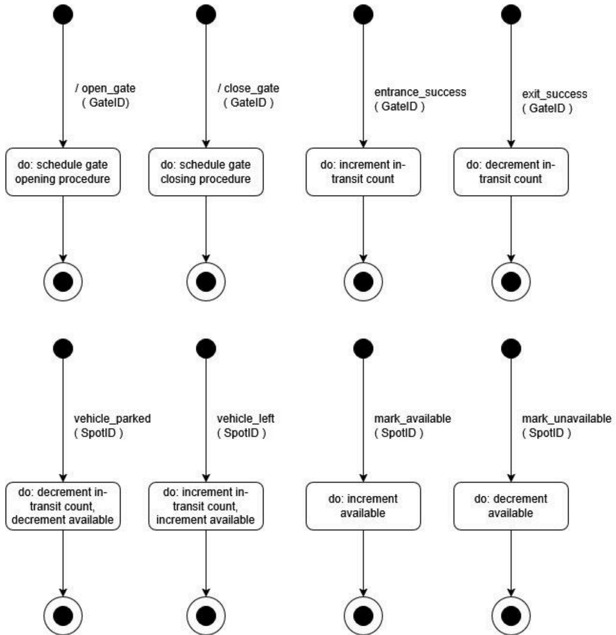
Figure 6: Central Controller Dynamic Diagram
