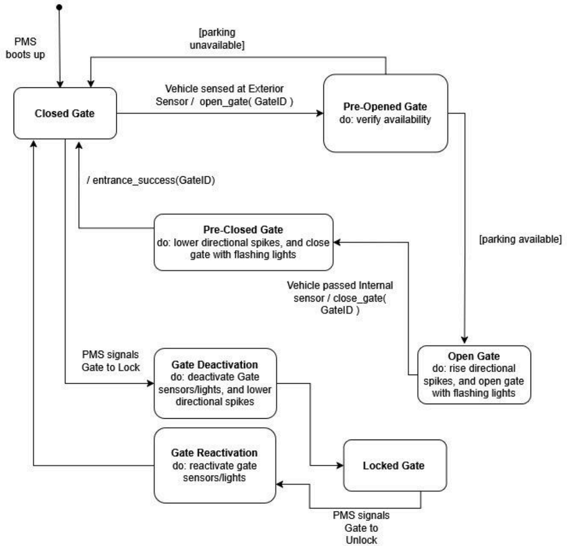
(4.a) Entrance Gate Dynamic Diagram
