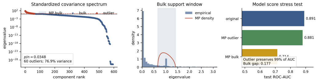
RMT Model Behavior: extra trees
