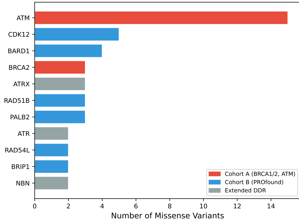
B) HRR Missense Variants by Gene
