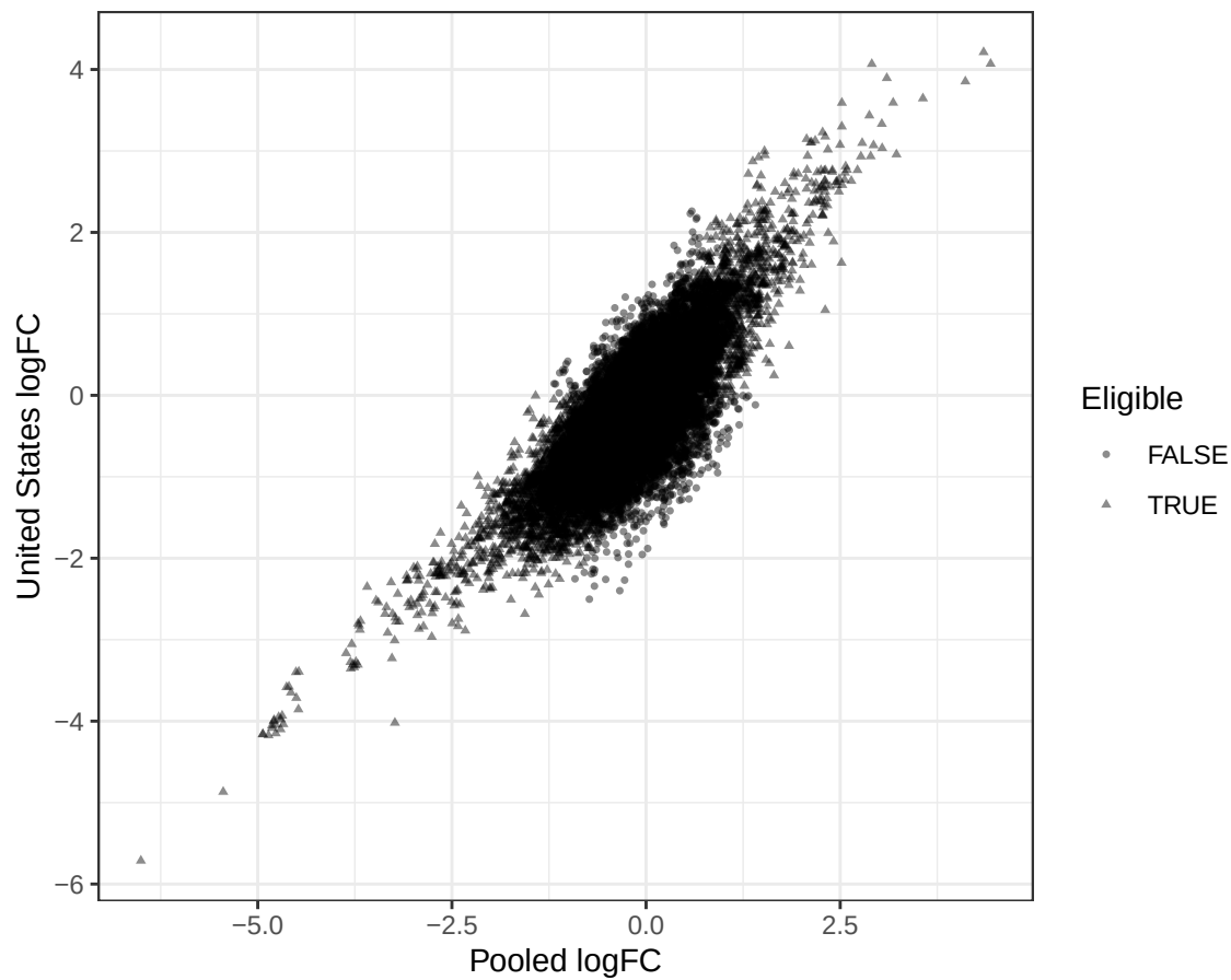
Pooled vs United States logFC with eligible stable features
